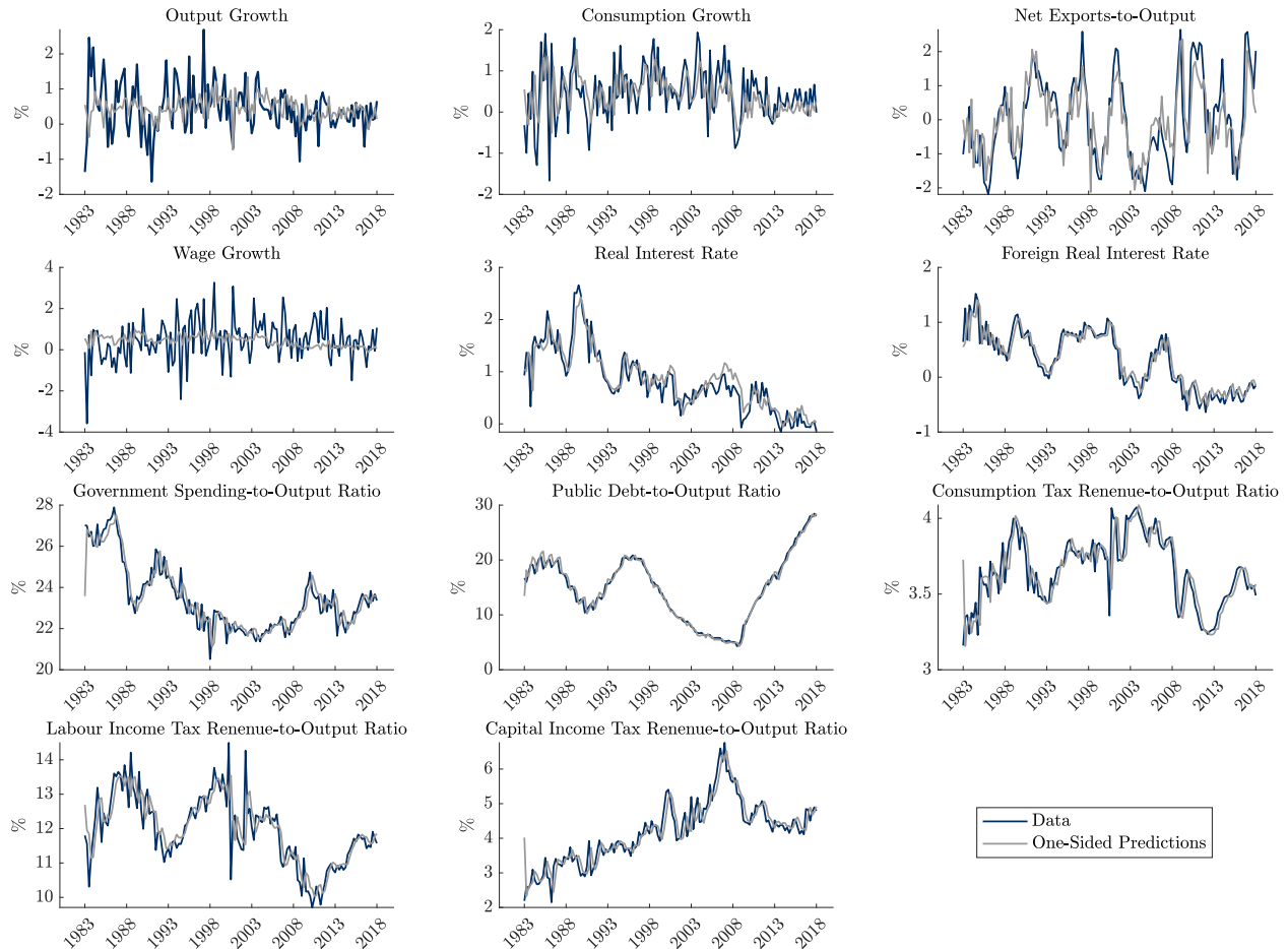
Figure 4: One-Sided Predictions and Data
